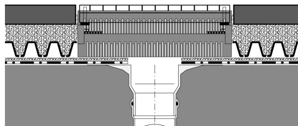
Terrace Grill TR-H 40 x 40 – 65 with Extension Piece
