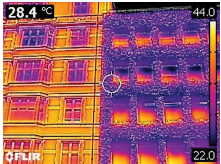
Thermal image showing the surface temperature of a green wall, central London Image: Gary Grant
