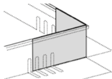
Creation of an internal corner with corner connector
