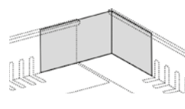
Creation of an external corner with corner connector
