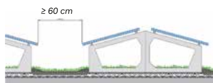
Solar Substructure Type "Saddle"
